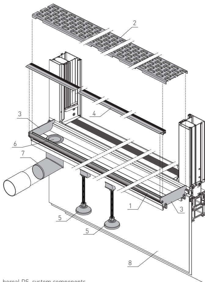
heroal DS, system components
