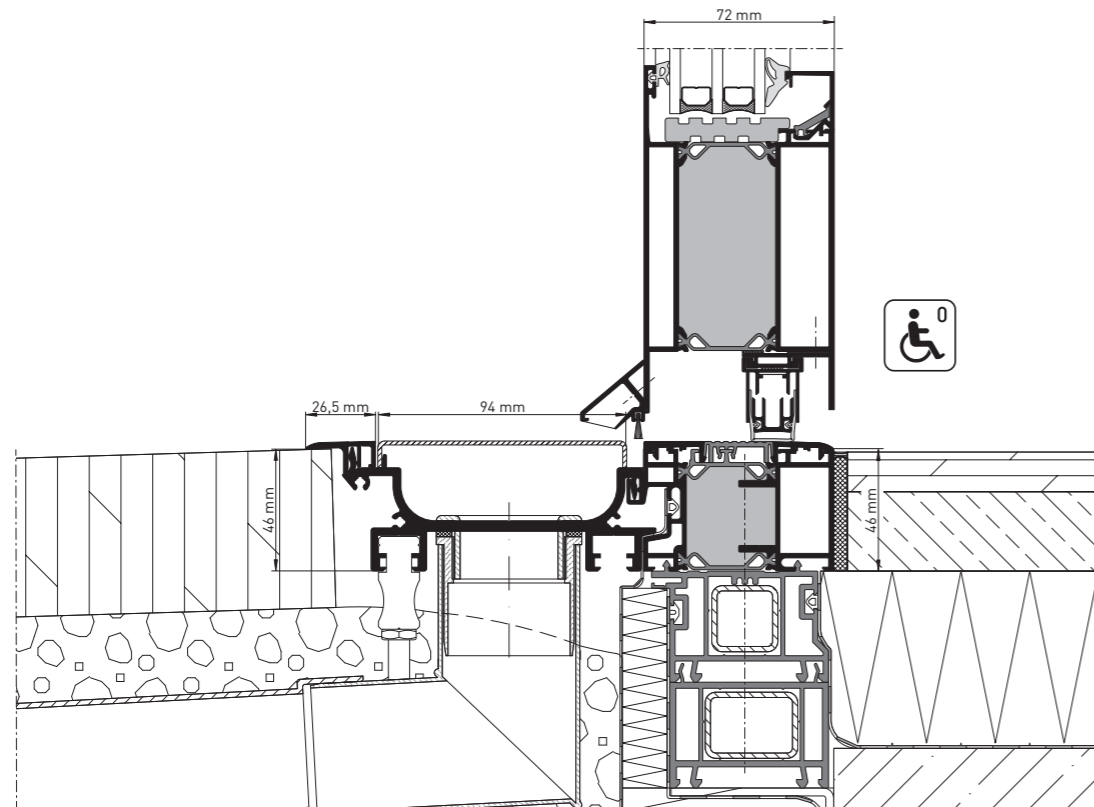
heroal D 72 with heroal DS, cross section
